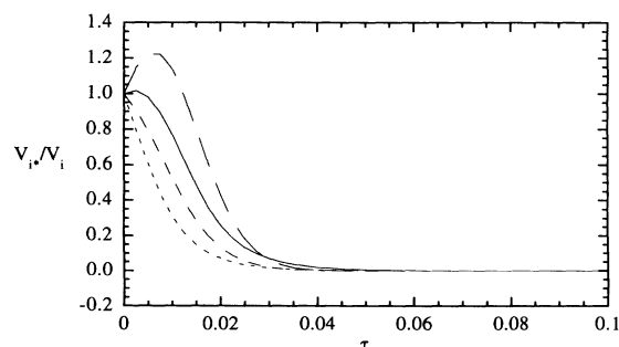
FIG. 2. The time evolution of the volume ratio V_{i*} / V_i for four different typical initial equilibrium phases from a constant internal energy simulation of 200 disks at H_0/N = 1.09161 , n=N/V=0.4 , and \gamma=1.0 .
